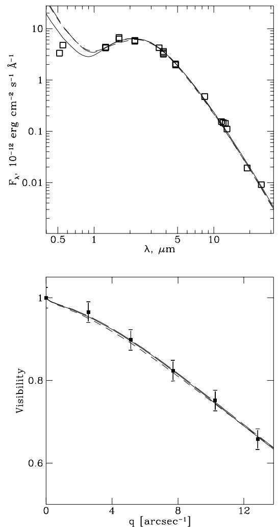
Fig. 3. Model SED corrected for interstellar extinction of A_V = 12.8 and 2.13 \mu\text{m} visibility function of WR 118 for the models M 1 (solid lines), M 2 (short-dashed lines), and M 3 (long-dashed lines) as given in Tables 1–2. The squares refer to the observations (see text).
