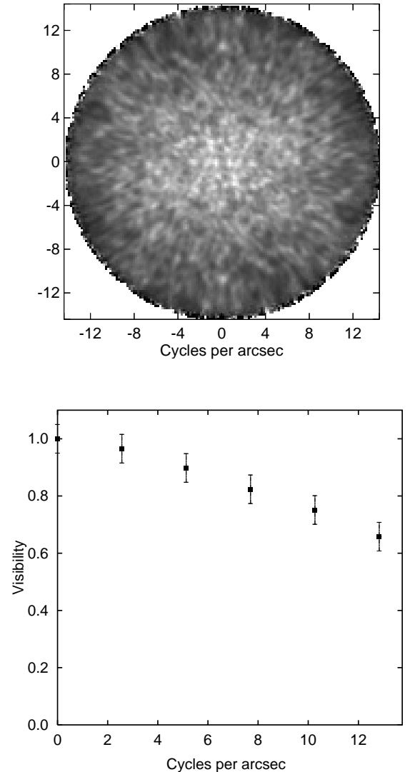
Fig. 1. Two-dimensional 2.13 \mu\text{m} visibility (top) and azimuthally averaged 2.13 \mu\text{m} visibility of WR 118 (bottom) shown up to the diffraction limit.
