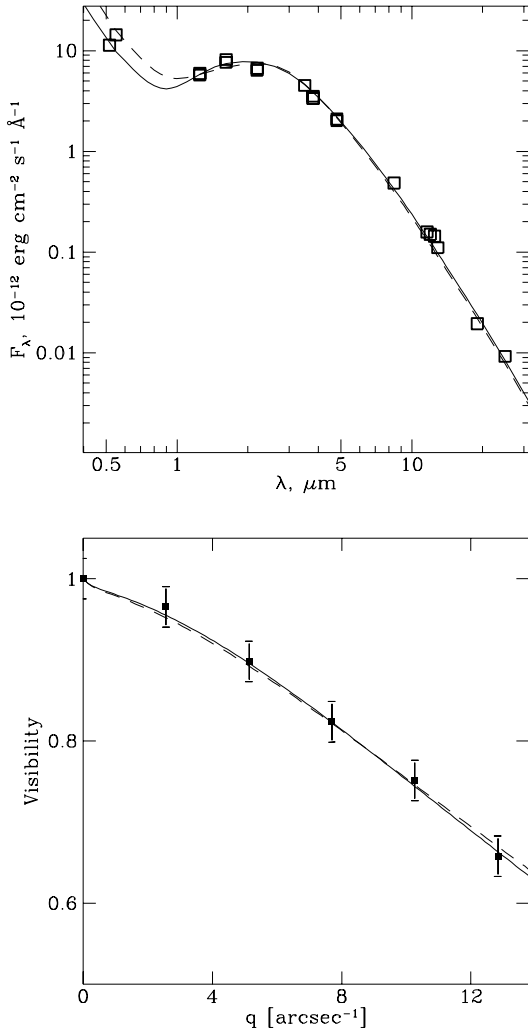
Fig. 4. Model SED corrected for interstellar extinction of A_V = 14.0 and 2.13 \mu\text{m} visibility function of WR 118 for the models M1.1 (solid lines) and M2.1 (short-dashed lines) as given in Tables 1–2. The squares refer to the observations (see text).
