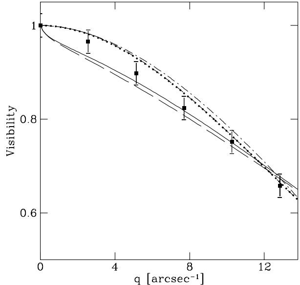
Fig. 2. 2.13 \mu\text{m} model visibility function of WR 118 for different optical depths and grain sizes for a dust-shell with r_{\text{in}} = 200 R_* together with the observed visibility. The dotted, short-dashed, dot-dashed, solid and long-dashed lines refer to \tau_V = 0.6 , a = 0.01 \mu\text{m} ; \tau_V = 0.6 , a = 0.10 \mu\text{m} ; \tau_V = 4.0 , a = 0.10 \mu\text{m} ; \tau_V = 4.0 , a = 0.38 \mu\text{m} ; and \tau_V = 0.6 , a = 0.38 \mu\text{m} , resp.
