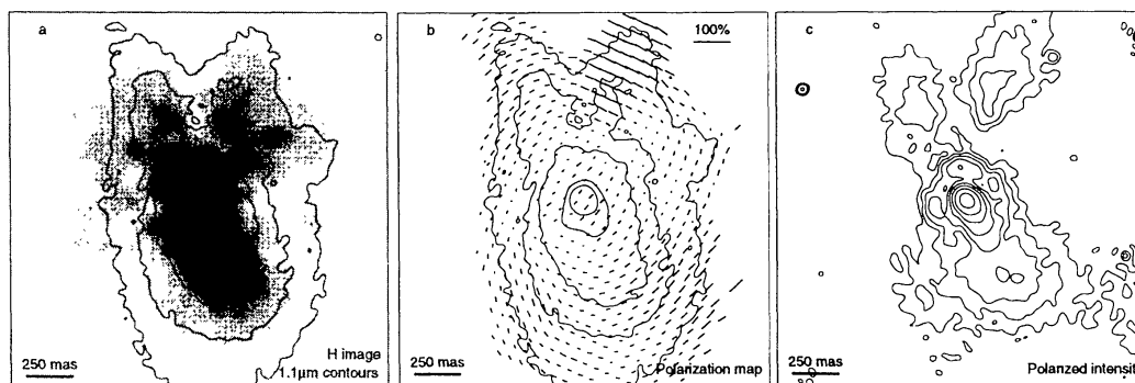
Fig. 3. a Superposition of the total intensity at 1.1 \mu\text{m} (contours are at 5.0, 4.2, 3.4, 1.8, and 1.0 mag relative to the peak) derived from the archival HST polarization data and the negative H speckle image. b 1.1 \mu\text{m} polarization map. The same contours as in frame a are shown. c Polarized intensity at 1.1 \mu\text{m} . The contours are plotted from 2.4 mag to 6.0 mag difference relative to the peak of the total intensity in steps of 0.6 mag. The structure of the polarization data at the position of B is affected by the diffraction pattern associated with A.
