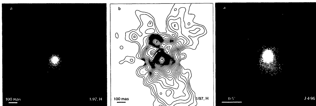
Fig. 2. a 70 mas resolution bispectrum speckle interferometry image of IRC +10216 in the H -band. North is up and east to the left. b Same as (a) as a contour image with denotations (A to G) of compact structures. Contours are at every 0.2 mag down to 5.0 mag relative to the peak. c J -band speckle reconstruction of IRC +10216 with 149 mas resolution.
