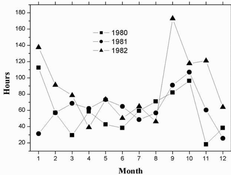
Figure 6: Distribution of clear night time in hours.
