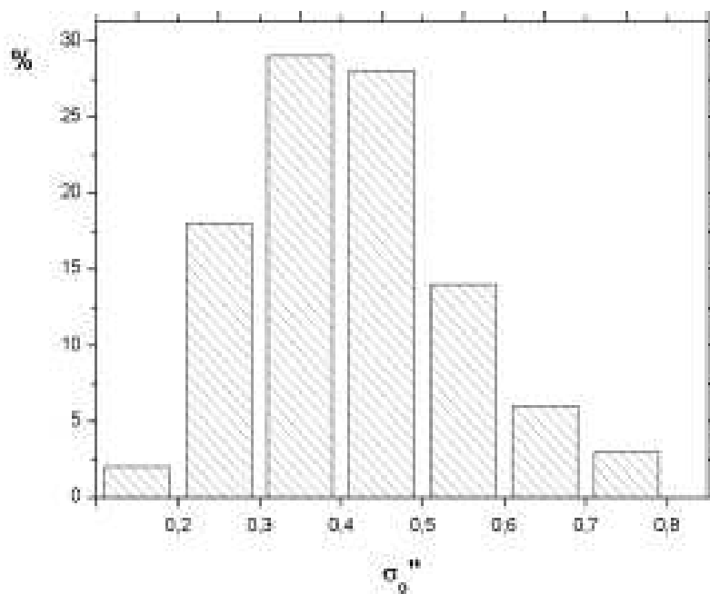
Figure 7: Distribution of flickering amplitudes.
