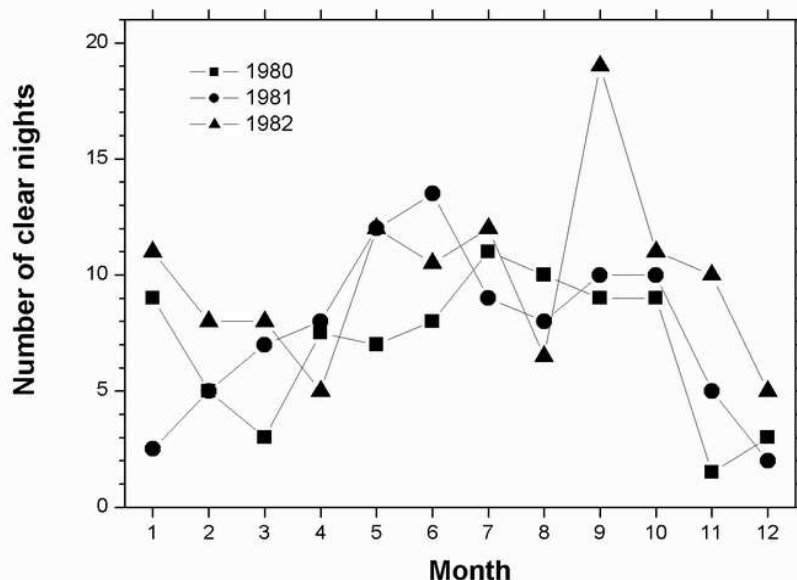
Figure 5: The number of clear nights in each month for 3 years.
